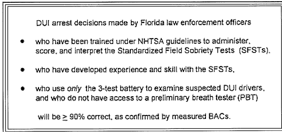
FIGURE 2 Study Hypothesis
